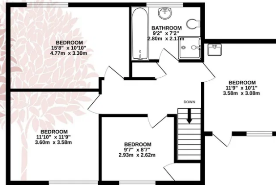
1ST FLOOR 681 sq.ft. (63.3 sq.m.) approx.
