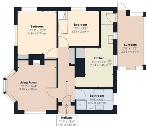
Floor 0
