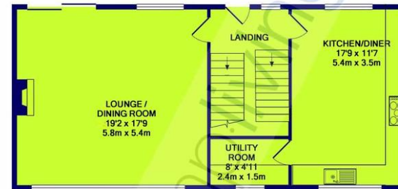
1ST FLOOR APPROX. FLOOR AREA 688 SQ.FT. (63.9 SQ.M.)
