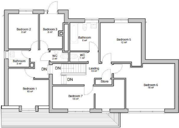
First Floor 1 : 100
