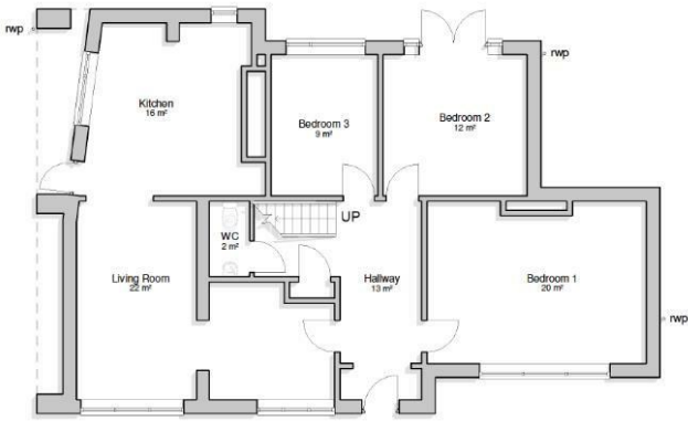
Ground Floor 1 : 100
