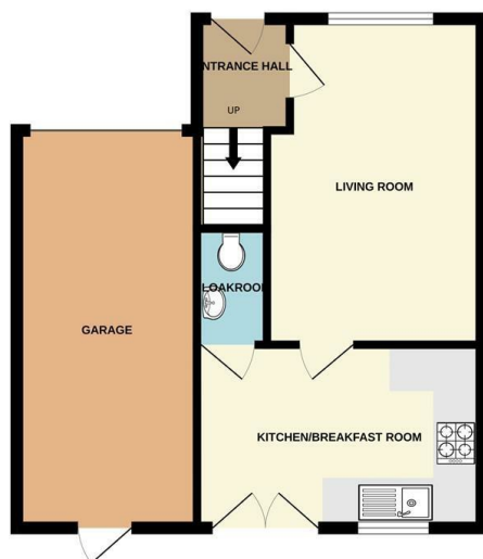
GROUND FLOOR 471 sq.ft. (43.8 sq.m.) approx.
