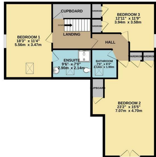
1ST FLOOR 923 sq.ft. (85.8 sq.m.) approx.
