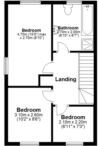
First Floor Approx. 39.1 sq. metres (420.5 sq. feet)
