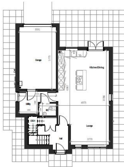
Ground Floor - Plan at A3 1:100 Plan at A1 1:50 Total internal area: 158m² (includes garage)
