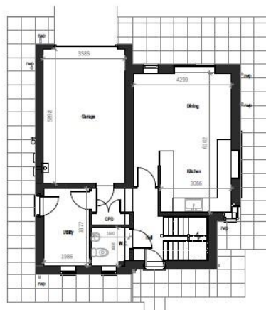
Ground Floor - Plan at A3 1:100 Plan at A1 1:50 Total internal area: 173m² (including garage)
