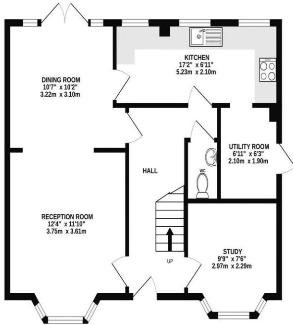
GROUND FLOOR 661 sq.ft. (61.4 sq.m.) approx.
