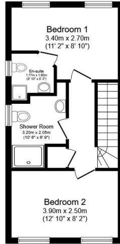
First Floor Floor area 34.4 sq.m. (370 sq.ft.)
