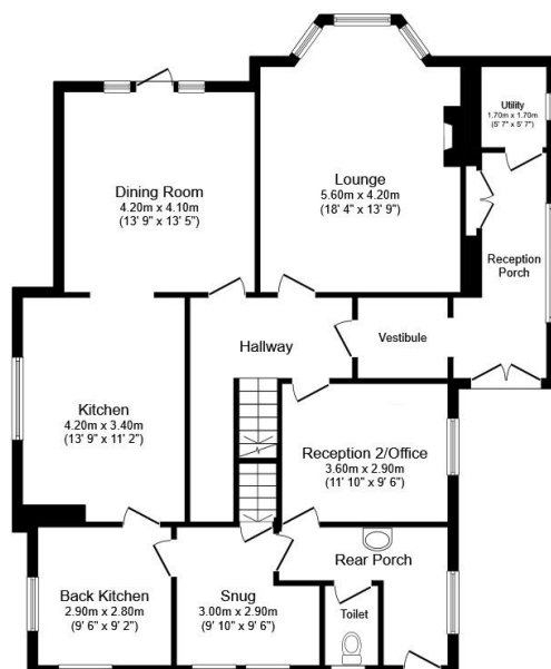
Ground Floor Floor area 119.5 m 2 (1,286 sq.ft.)
