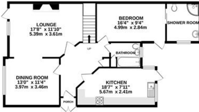
GROUND FLOOR 1109 sq.ft. (102.0 sq.m.) approx.
