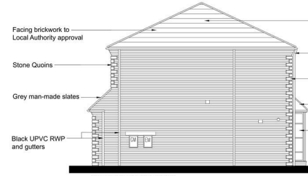
SOUTH ELEVATION (SIDE)
