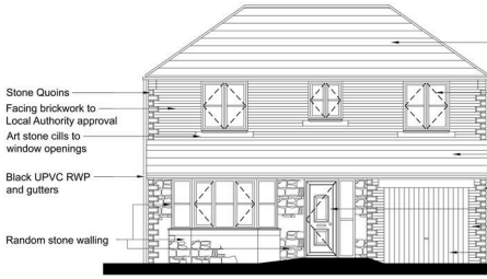
WEST ELEVATION (FRONT)
