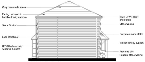
NORTH ELEVATION (SIDE)
