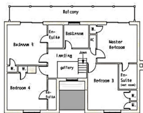
First Floor Plan 1:188
