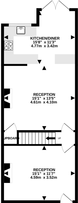
GROUND FLOOR 551 sq.ft. (51.2 sq.m.) approx.
