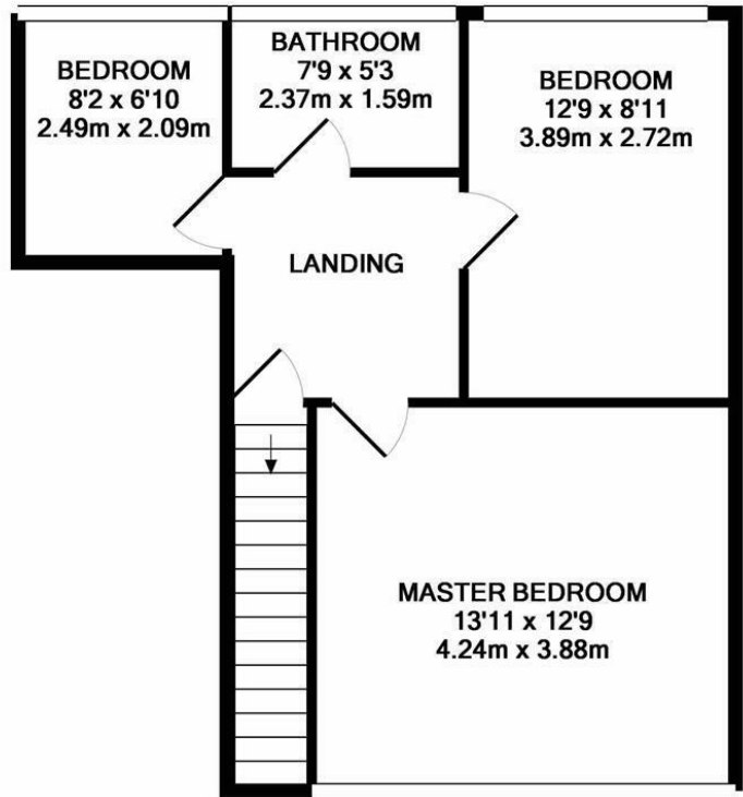
1ST FLOOR APPROX. FLOOR AREA 482 SQ.FT. (44.8 SQ.M.)
