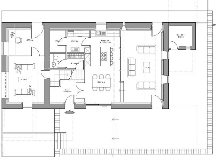
Approved Ground Floor
