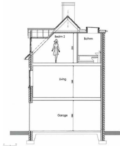
Project Proposed New Dwelling at: Waters Edge, Mill Road, Meole Shrewsbury, SY3 9JT Drawing Proposed Section scale 1:50 paper size A3 A 23.11.18 Rr
