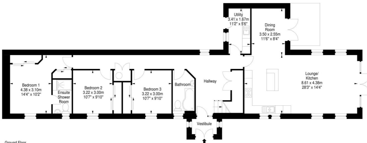
Ground Floor
