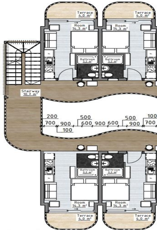
17.5m 2 floor plan
