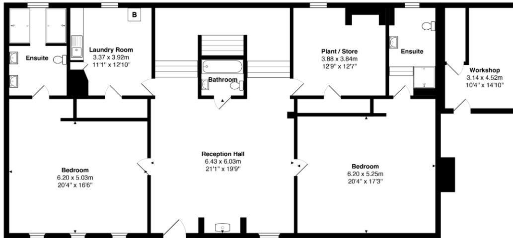
Ground Floor Area: 209.2 m 2 ... 2252 ft 2
