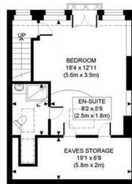
SECOND FLOOR GROSS INTERNAL FLOOR AREA WITH EAVES STORAGE 501 SQ FT FLOOR AREA WITHOUT EAVES STORAGE 376 SQ FT
