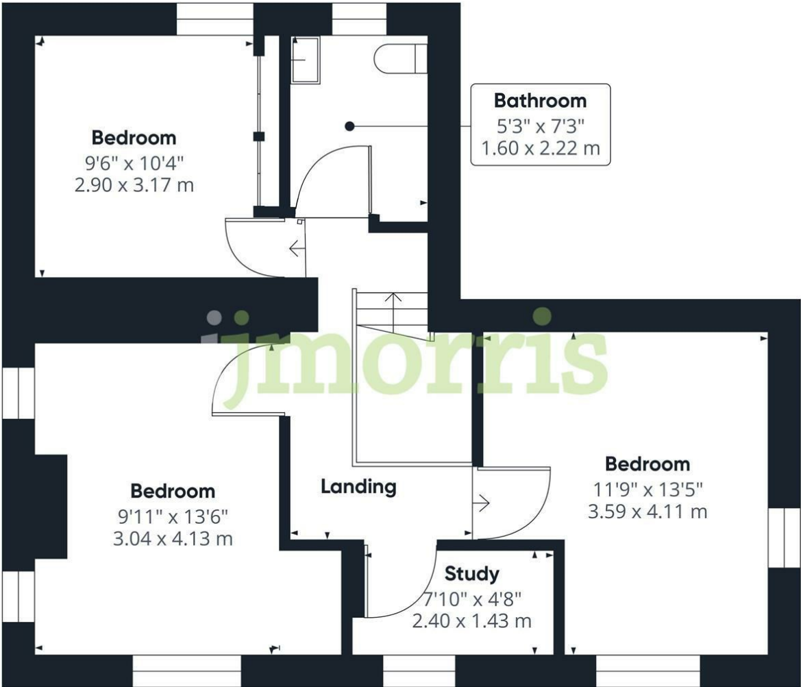
Floor 1 Building 1
