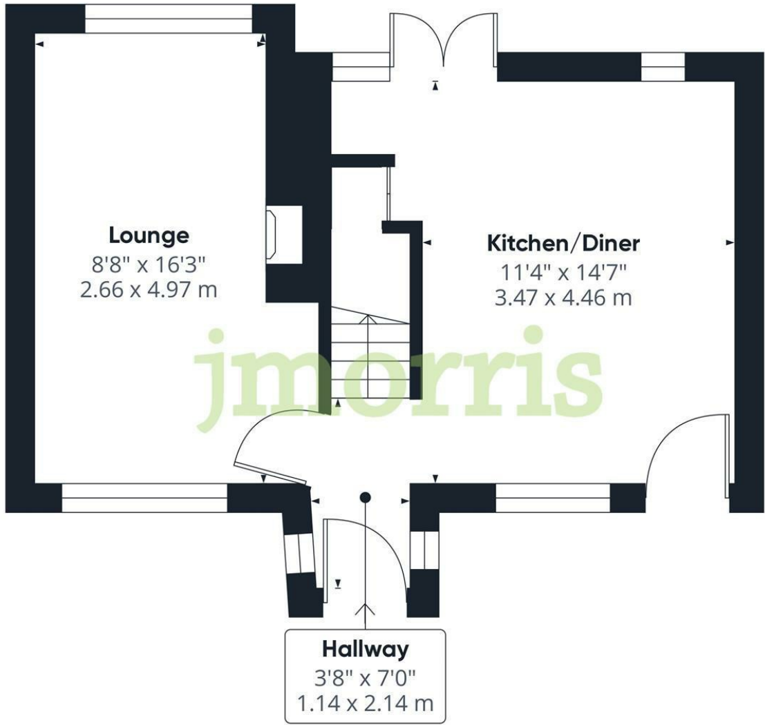
Floor 0
