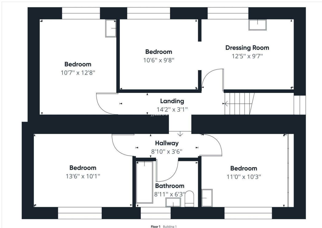
Floor 1 Building 1
