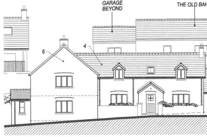
FRONT ELEVATION 1:200
