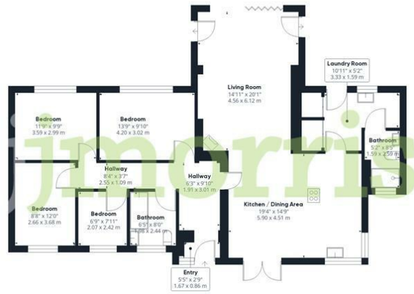
Floor 0 Building 1
