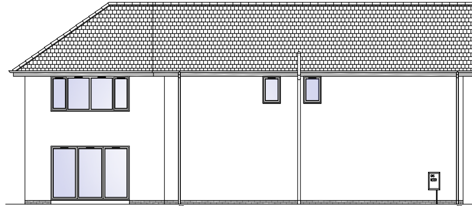
Rear Elevation
