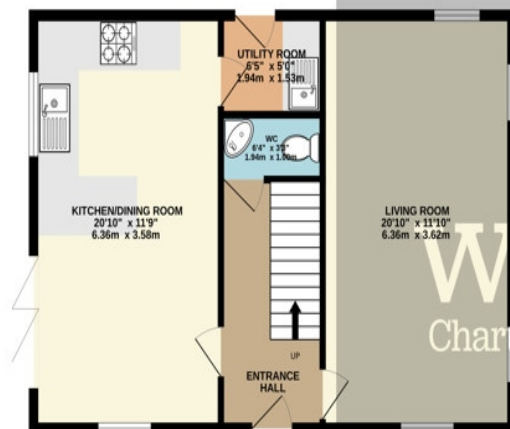
GROUND FLOOR 625 sq.ft. (58.1 sq.m.) approx.
