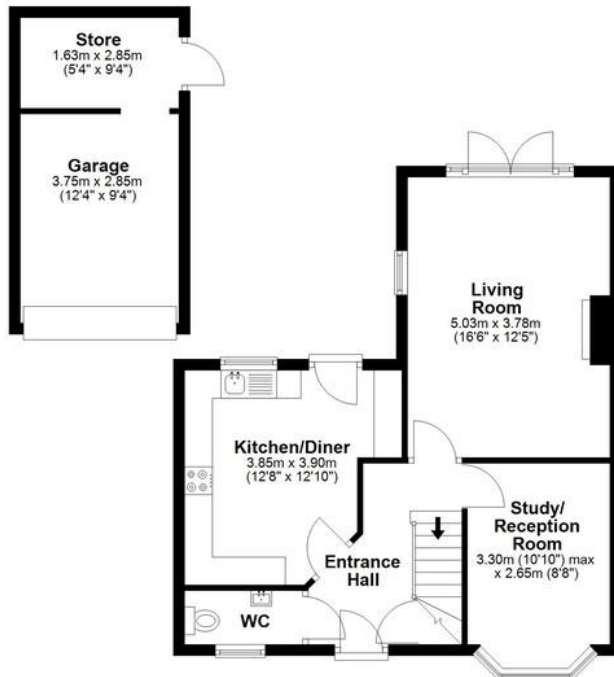
Ground Floor Approx. 67.2 sq. metres (723.0 sq. feet)
