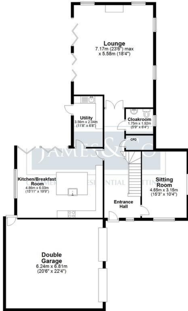
Ground Floor Approx. 156.5 sq. metres (1684.8 sq. feet)
