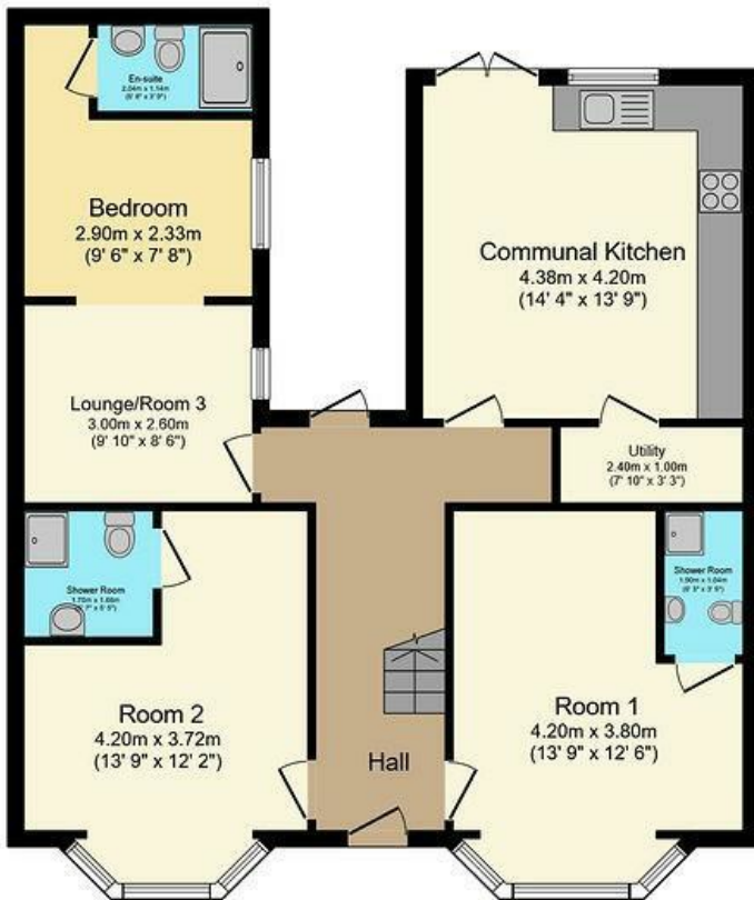
Ground Floor Floor area 87.6 sq.m. (943 sq.ft.)
