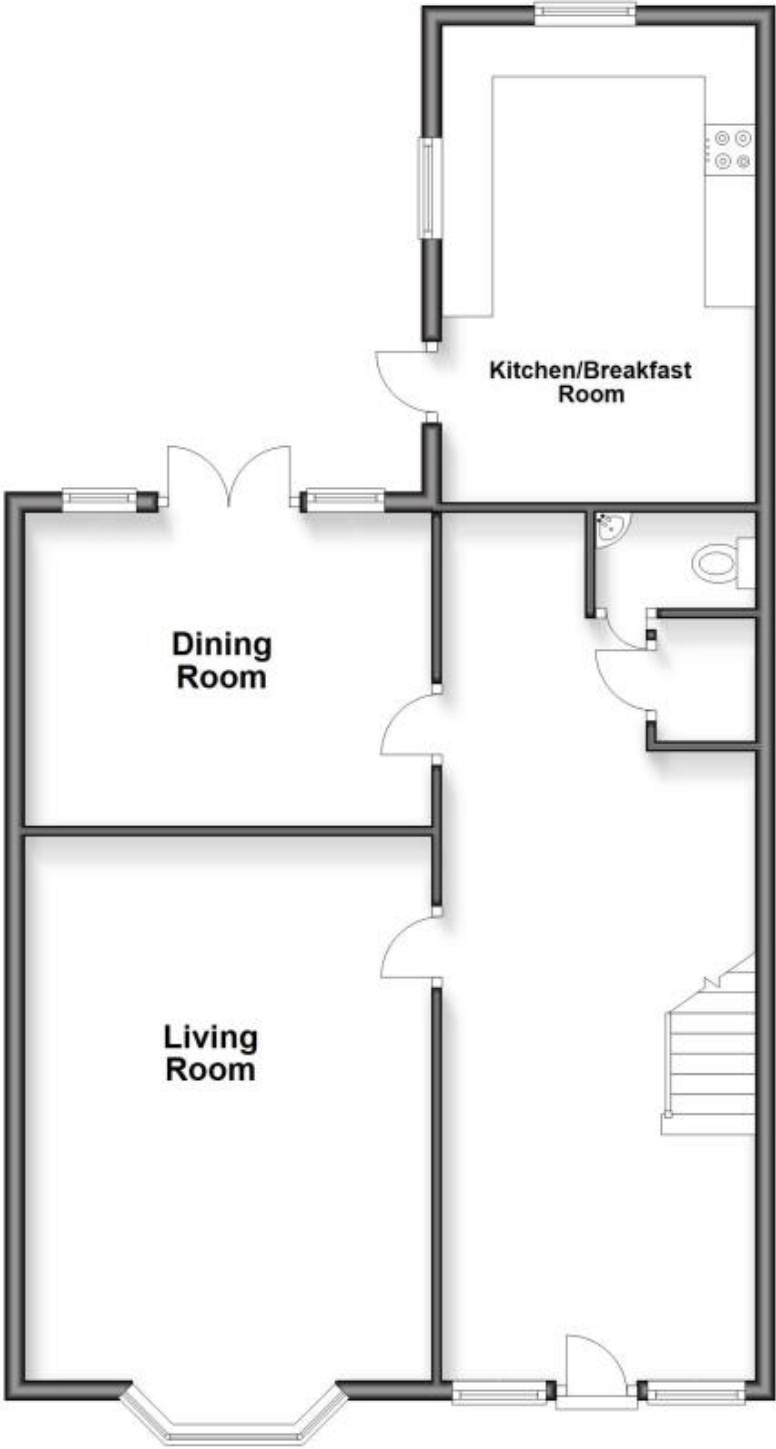
Ground Floor
