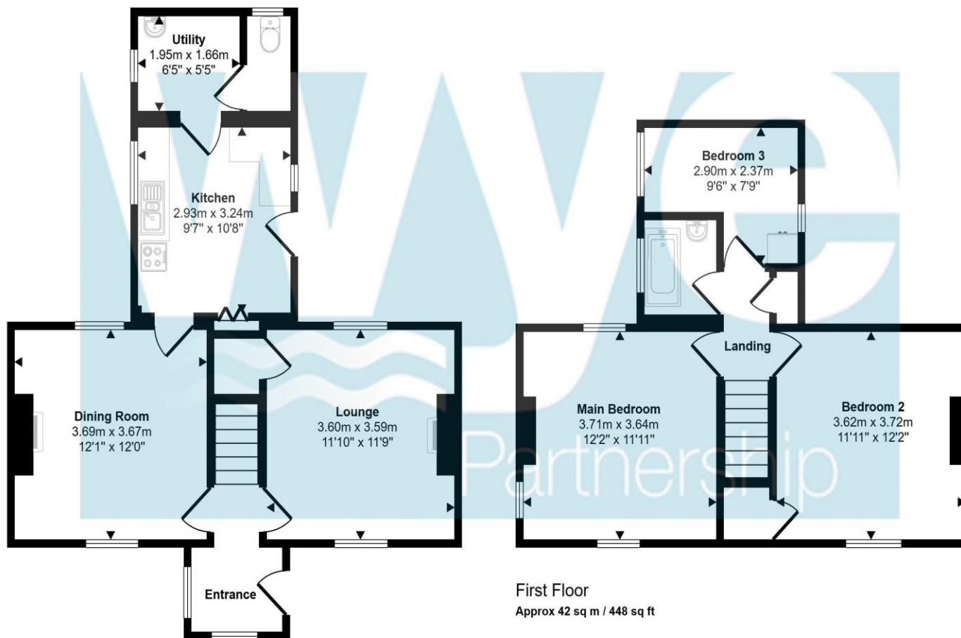
Ground Floor Approx 49 sq m / 532 sq ft
