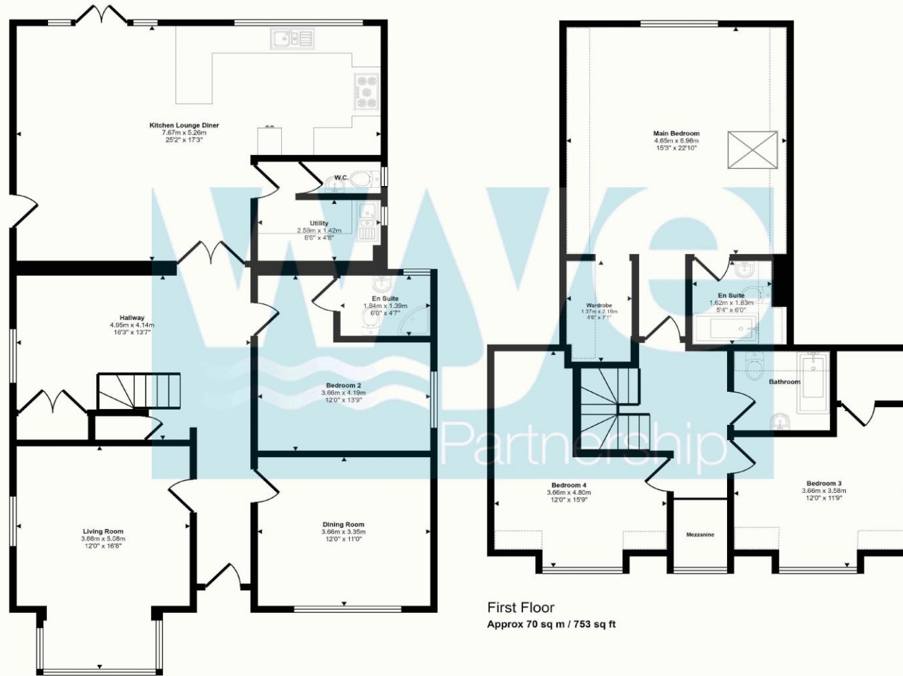
Ground Floor Approx 107 sq m / 1156 sq ft
