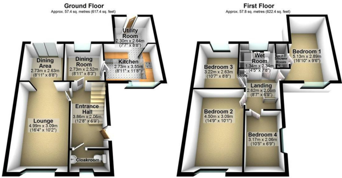
Total area: approx. 115.2 sq. metres (1239.8 sq. feet)
