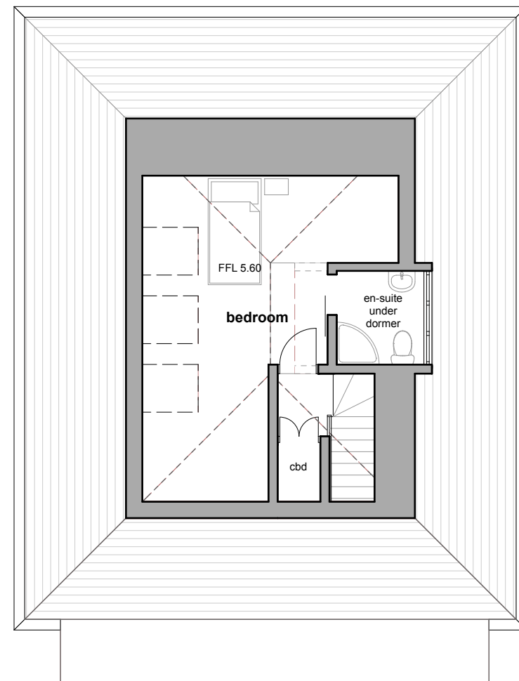
Proposed Loft Plan @ 1:100
