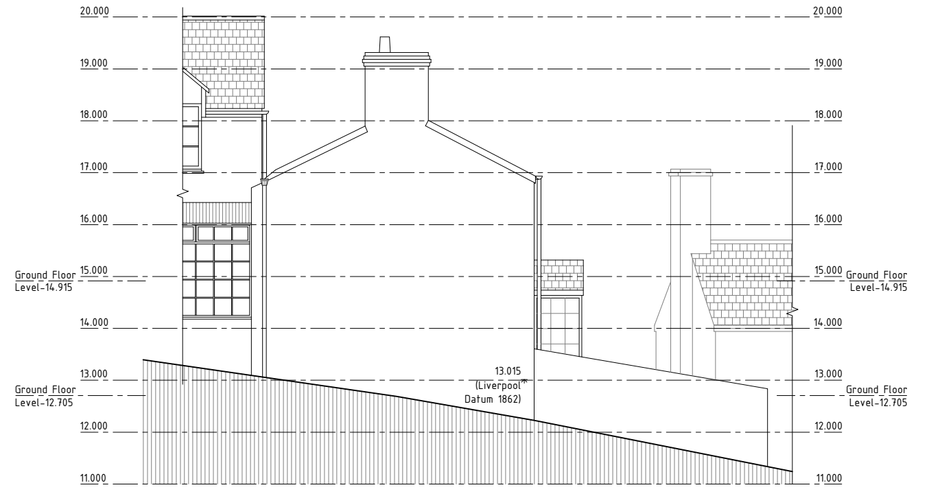
West Elevation
