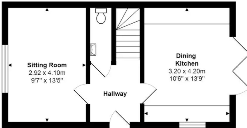
Ground Floor Area: 35.8 m 2 ... 385 ft 2
