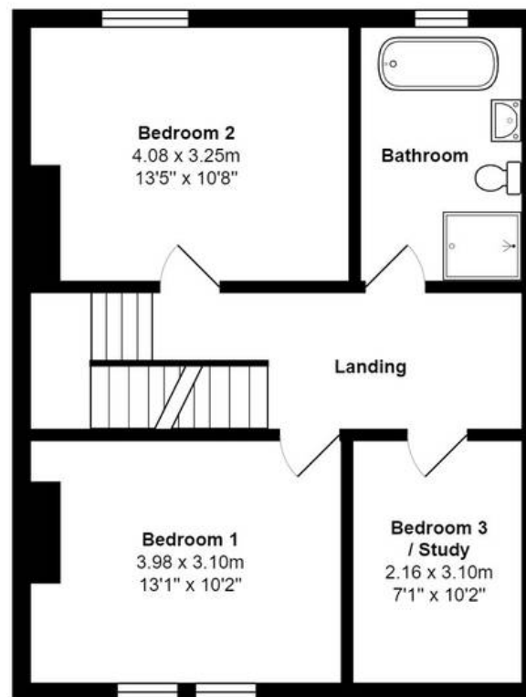
First Floor Area: 53.0 m 2 ... 570 ft 2
