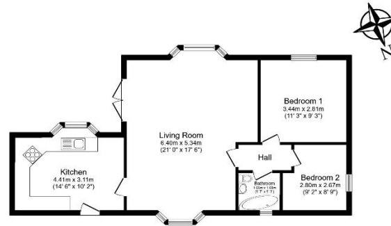
Total floor area 72.8 sq.m. (784 sq.ft.) approx This floor plan is for illustrative purposes only. It is not drawn to scale. Any measurements, floor areas (including any total floor area), openings and orientation are approximate. No details are guaranteed, they cannot be relied upon for any purpose and they do not form part of any agreement. No liability is taken for any error, omission or misstatement. A party must rely upon its own inspection(s). Powered by www.bodagert.com
