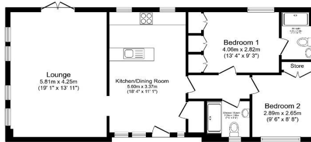
Total floor area 76.4 sq.m. (822 sq.ft.) approx This floor plan is for illustrative purposes only. It is not drawn to scale. Any measurements, floor areas (including any total floor area), openings and orientation are approximate. No details are guaranteed, they cannot be relied upon for any purpose and they do not form part of any agreement. No liability is taken for any error, omission or misstatement. A party must rely upon its own inspection(s). Powered by www.houseagent.com
