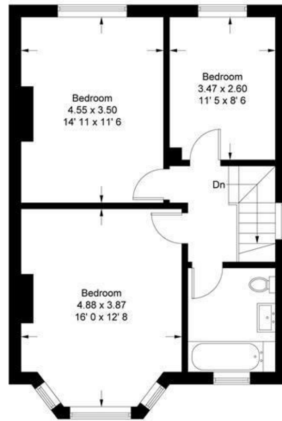
First Floor 607 sq ft / 56.4 sq m
