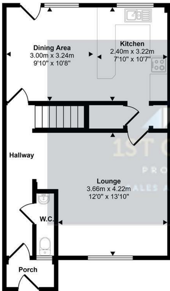
Ground Floor Approx 49 sq m / 528 sq ft
