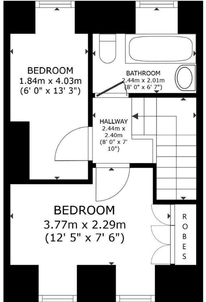
FLOOR 2
