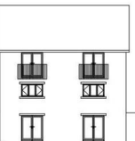
REAR ELEVATION
