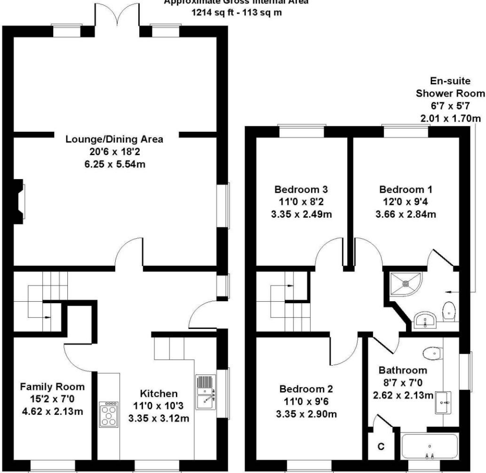
GROUND FLOOR
