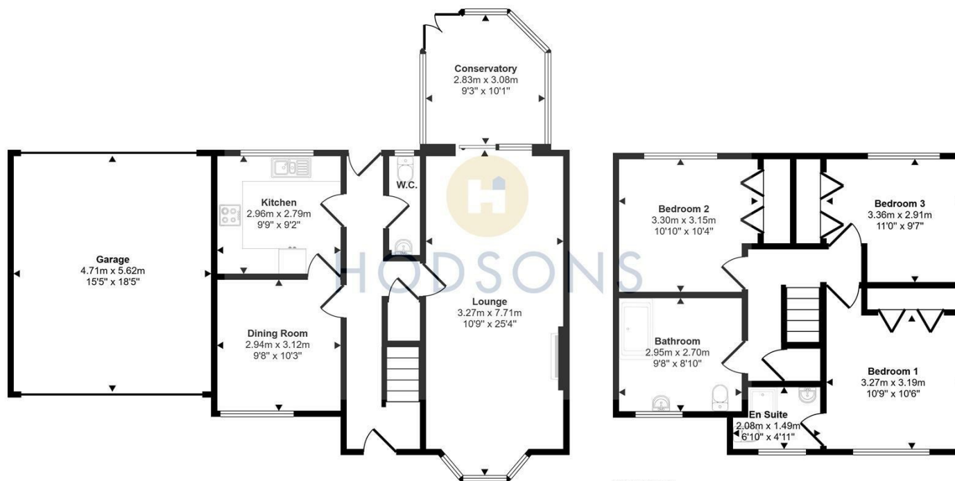
Ground Floor Approx 92 sq m / 987 sq ft
