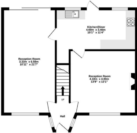
Ground Floor 56.3 sq.m. (606 sq.ft.) approx.
